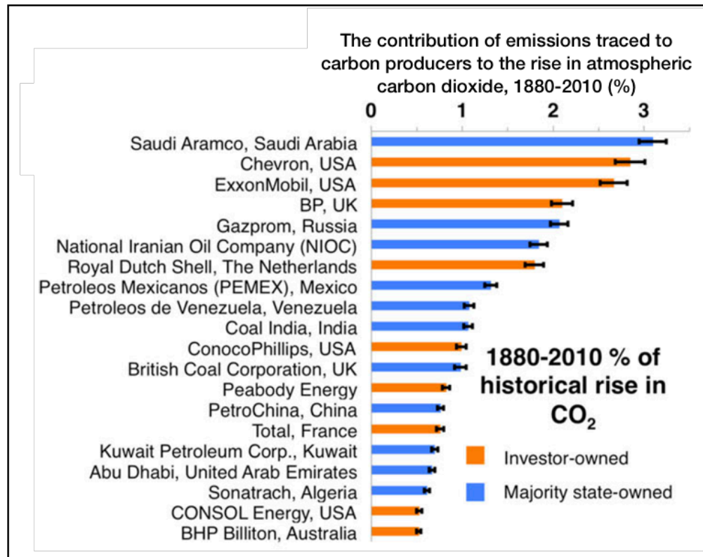
Figure 6. Top twenty investor- & state-owned entities and attributed CO 2 emissions. Emissions from these companies contributed about 27.2 ( \pm 2.9 ) % of increase in cumulative atmospheric CO 2 between 1880 and 2010. Figure modified from: Ekwurzel, B., et al. The Rise in Global Atmospheric CO 2 , Surface Temperature, and Sea Level from Emissions Traced to Major Carbon Producers , 144(4) Climatic Change 579–590 (2017).
